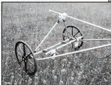
Non-magnetic MagCart for 1 to 5 sensors improves data quality and target analysis for precise mapping of sites.
