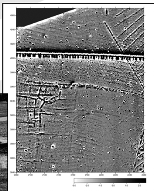
Cesium magnetometer data of a "Sub-Roman" settlement with enclosures, ridge and furrow field patterns. (Data courtesy of Archaeophysics)
